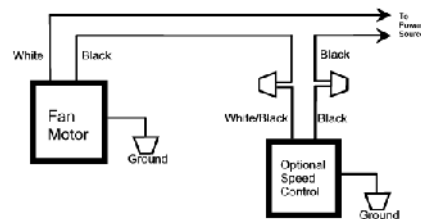
Figure 2 – Wiring
