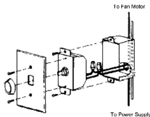
Figure 1 – Mounting
